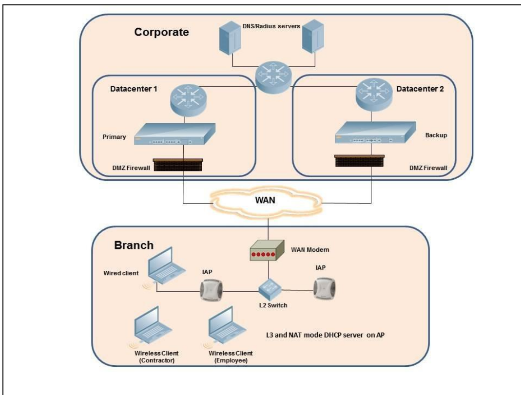
Figure 136 Scenario 3—IPSec: Multiple Datacenter Deployment with Primary and Backup Controllers for Redundancy
