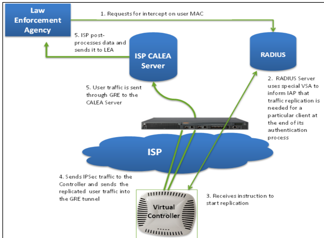
Figure 94 IAP to CALEA Server through VPN
