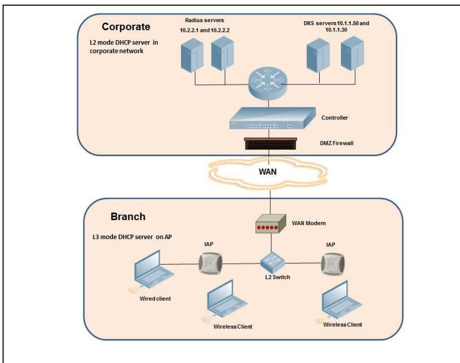
Figure 134 Scenario 1—IPSec: Single datacenter Deployment with No Redundancy
