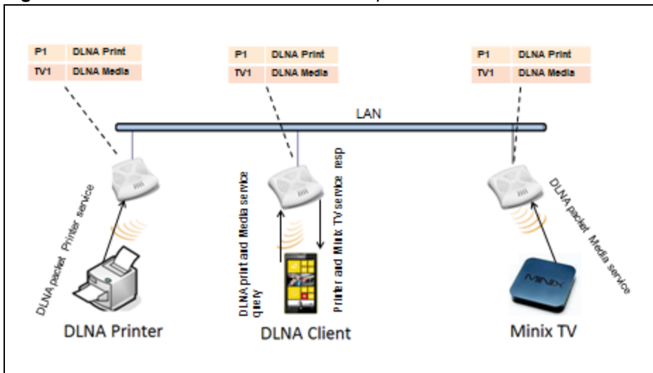
Figure 86 DLNA UPnP Services and AirGroup Architecture
