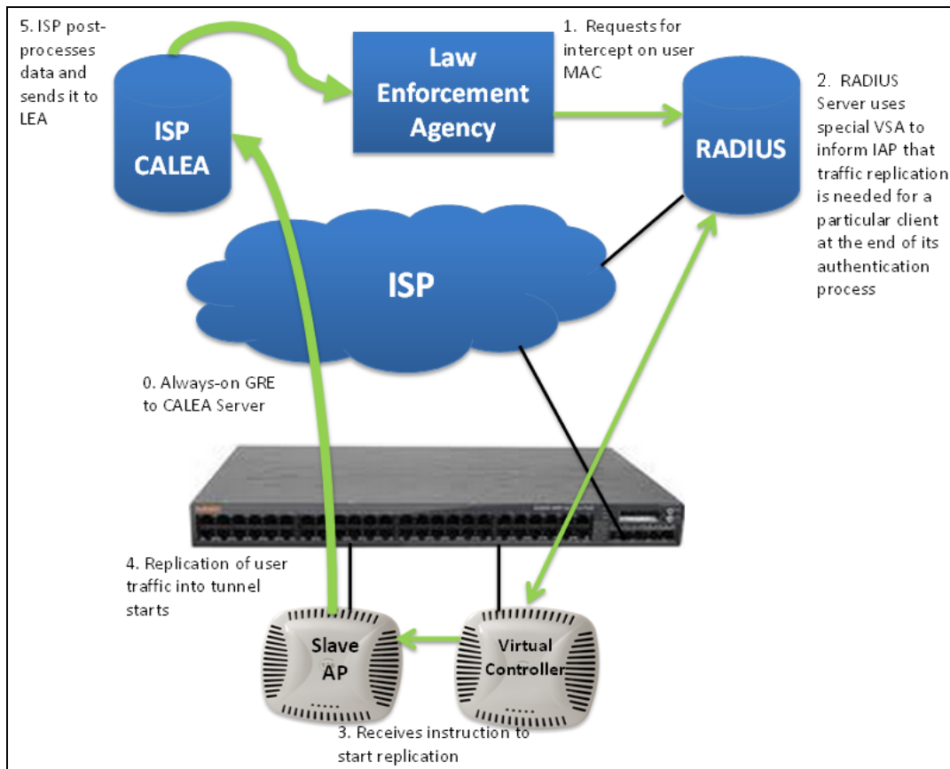
Figure 93 IAP to CALEA Server
