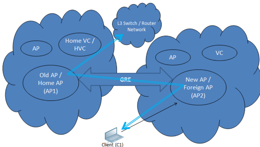
Figure 113 Routing of traffic when the client is away from its home network
